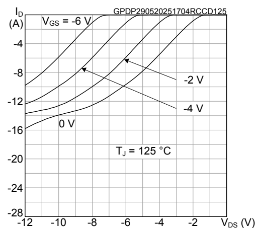
Figure 16. Typical diode reverse conduction characteristics ( T_J = 125^\circ C )
