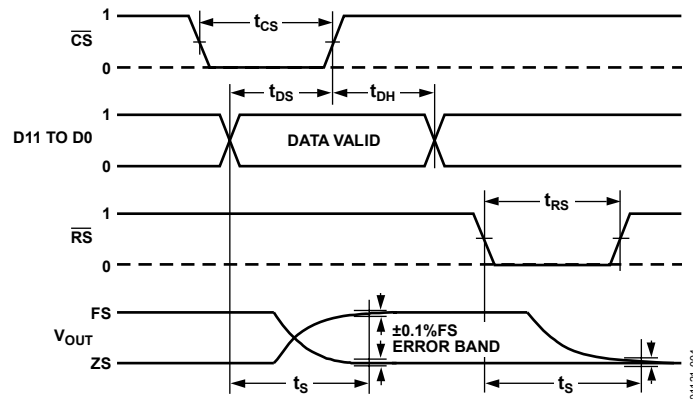
Figure 2. Timing Diagram
