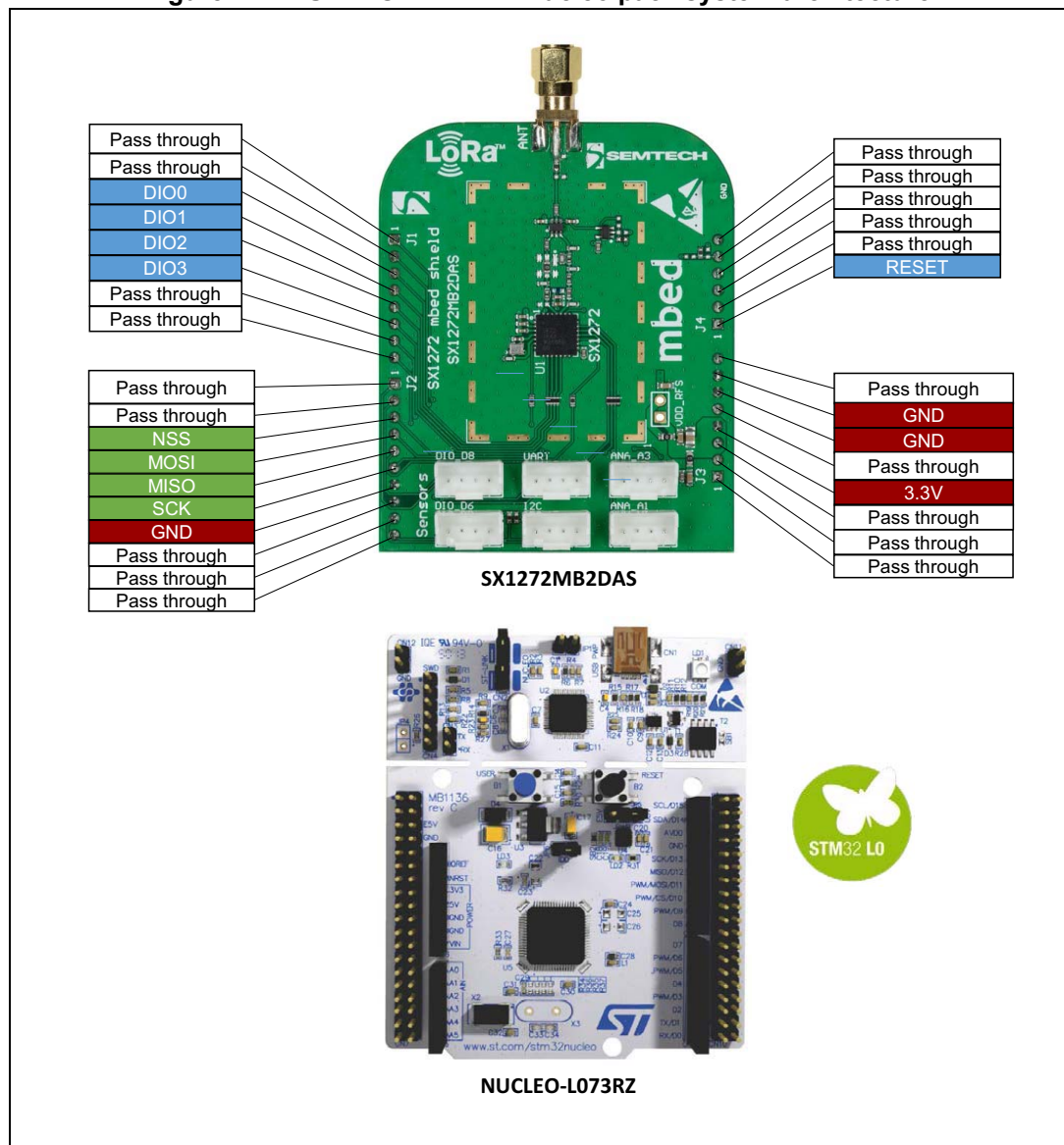
Figure 2. P-NUCLEO-LRWAN1 Nucleo pack system architecture
