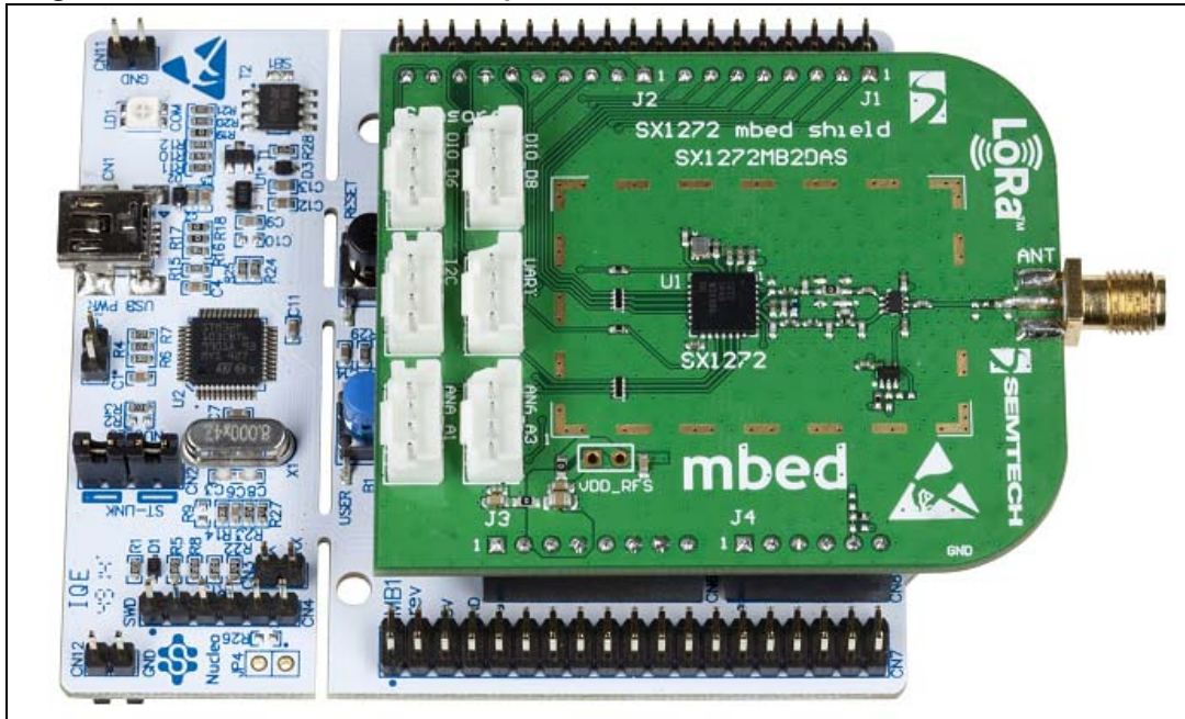
Figure 3. SX1272MB2DAS LoRa expansion board and NUCLEO-L073RZ assembled
