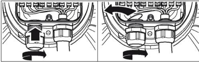
Fig. 2: Cable gland opening
