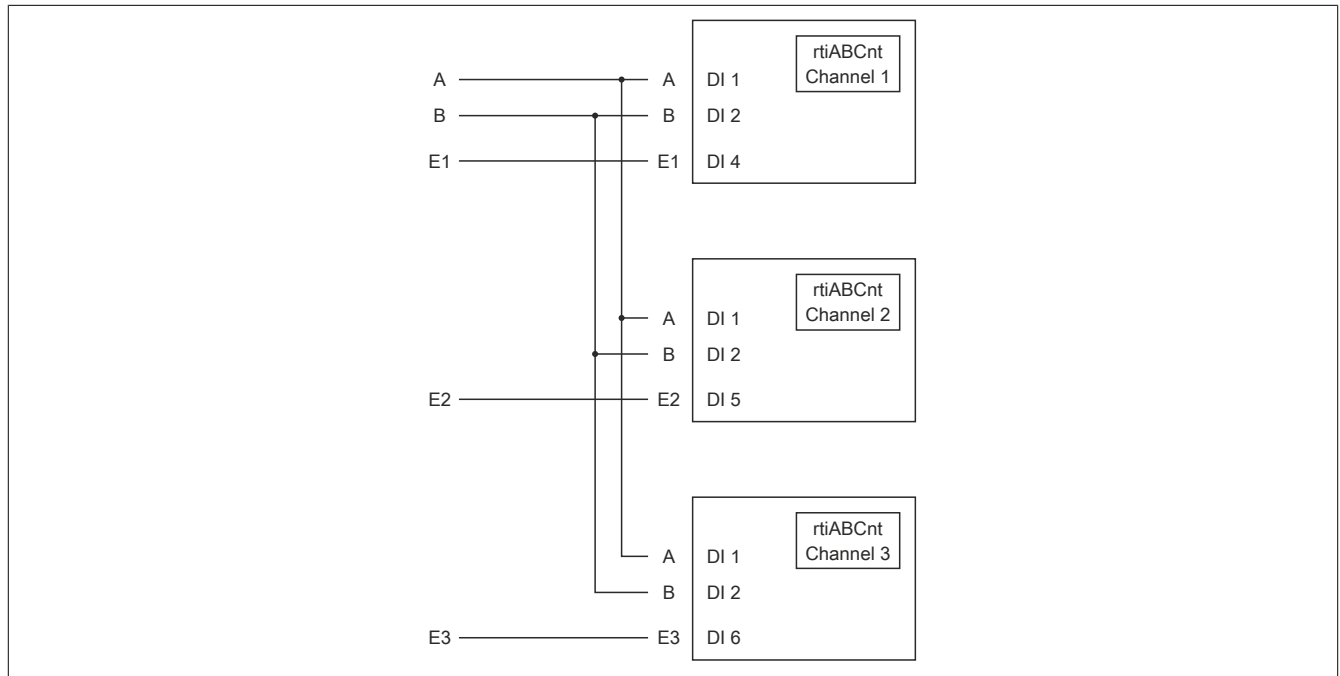
Figure 11: Schematic diagram of input signals for rtiABCnt
