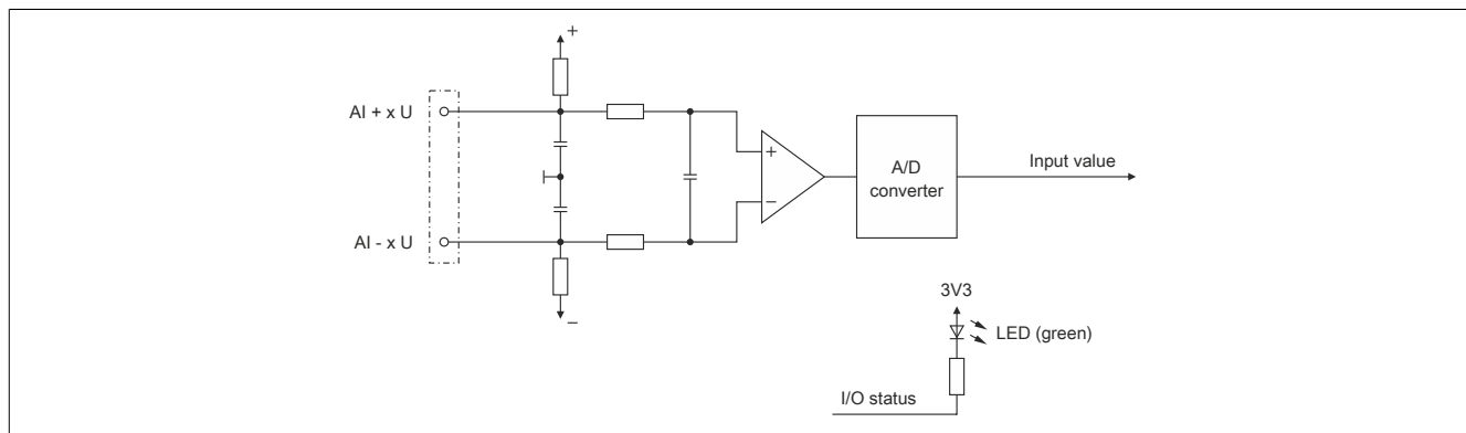
Figure 8: Input circuit diagram of the analog input (X2)
