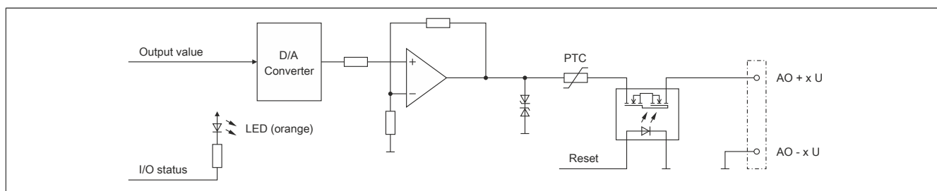
Figure 9: Output circuit diagram of the analog output (X2)
