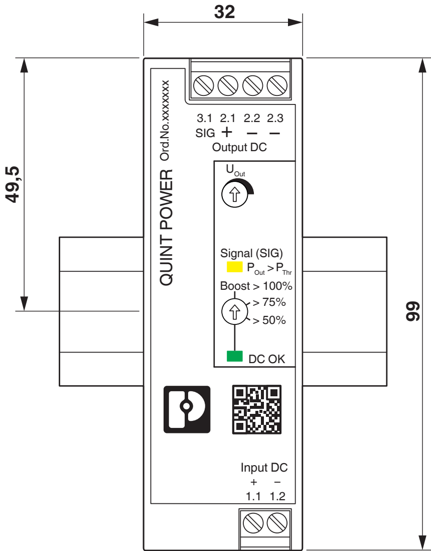
Dimensional drawing
