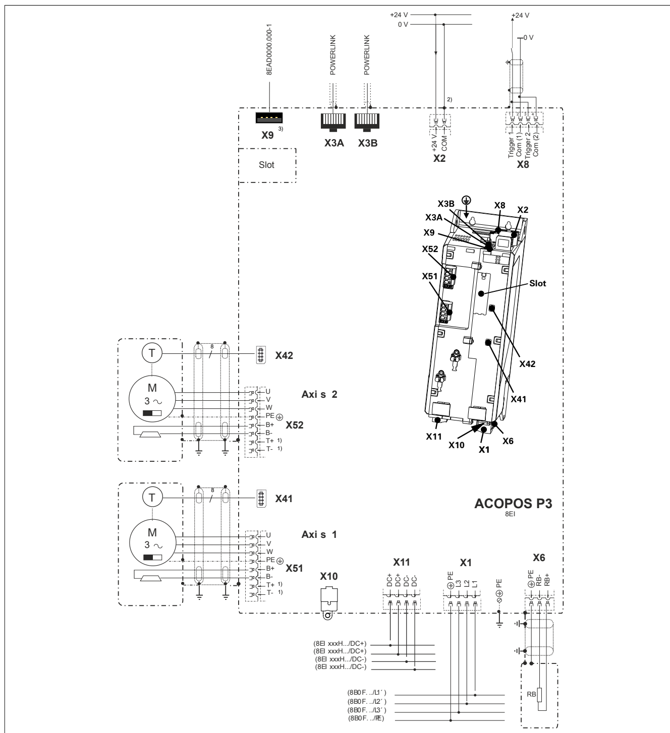
Figure 4: Mains input voltage - 3x 200 to 480 VAC
