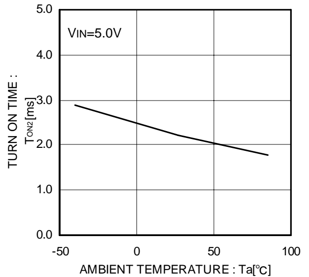
Figure 64. Output turn on time
