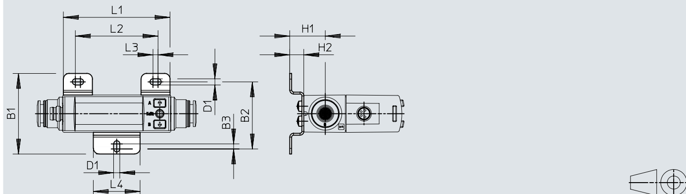
Dimensions – Wall mounting SAMH-FH-W
