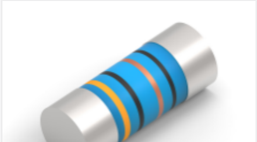
TE Part #2176314-4 MELF SMA_A 180R 0.1% 15PPM 0102 0.3W
