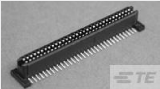
TE Part #5146893-2 1FHR,84,30A/S,S,C,S08,09,10
