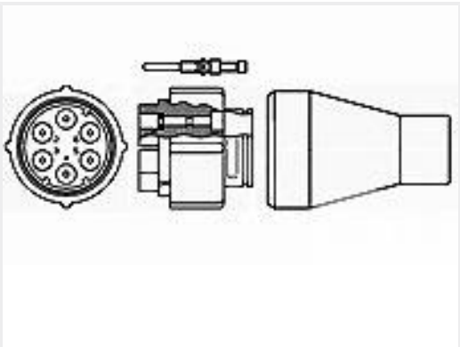
TE Part #863024-2 LGH PLUG ASSY HV 7 PIN
