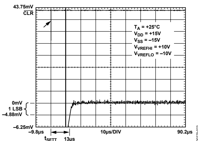
Figure 22. Negative Settling Time ( \pm 15\text{ V} )
