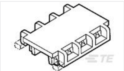
TE Part #643077-5 05P MTA100 MOLDED COVER F/T
