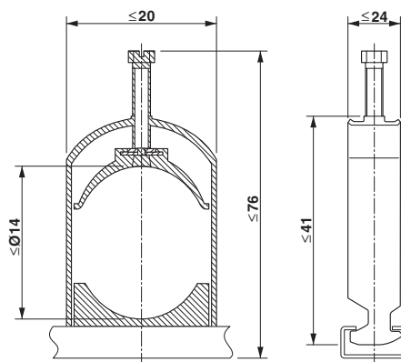
Dimensioned drawing
