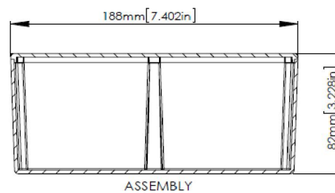
ASSEMBLY
