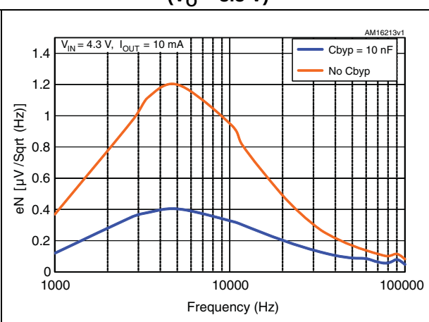
Figure 23. Output noise vs. frequency ( V_O = 3.3 V)
