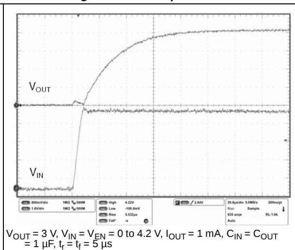
Figure 31. Startup transient
