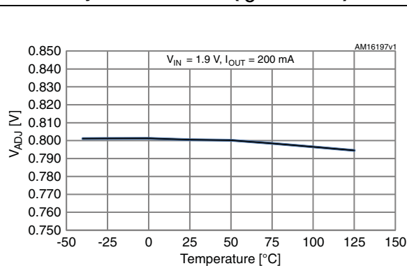
Figure 7. Output voltage vs. temp. for adjustable version ( I_O = 200\ \text{mA} )
