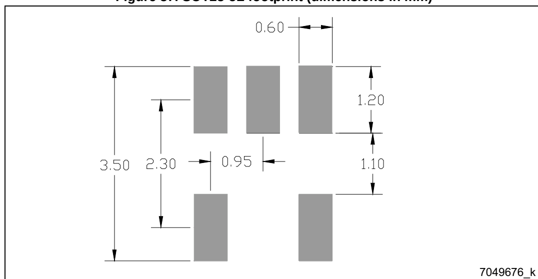
Figure 37. SOT23-5L footprint (dimensions in mm)
