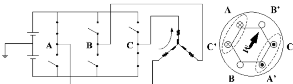
Figure 2: Conduction interval of 120-degree commutation.
