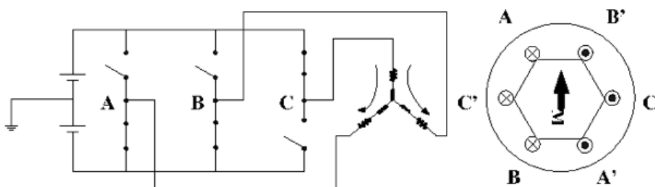
Figure 3: Conduction interval of 180 degree commutation.
