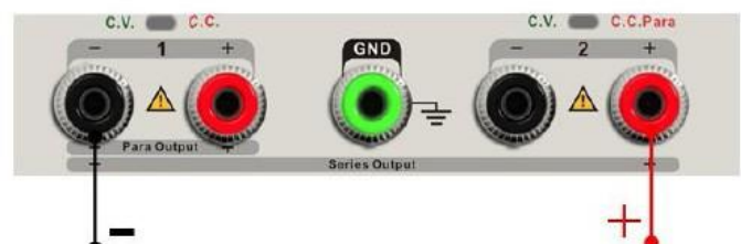
Series connection
