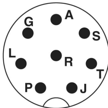
Connector pin assignment for M12 plug-in connection, 8-pos.
