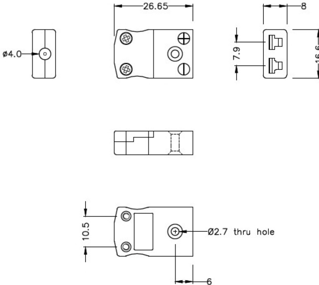
Miniature in-line Socket (dimensions in mm)
