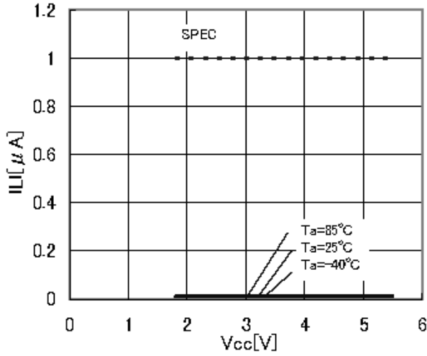
Figure 6. Input Leak Current ILI (SCL, WP)
