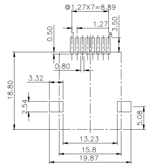
Recommended PCB Layout (Top side)
