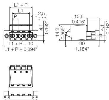
Dimensioned drawing
