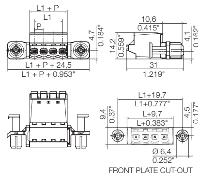
FRONT PLATE CUT-OUT
