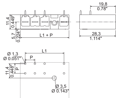
Dimensioned drawing
