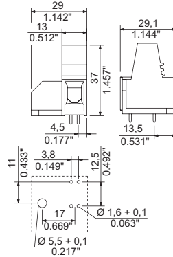
Dimensioned drawing
