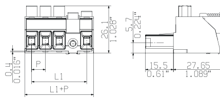
Dimensioned drawing
