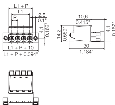
Dimensioned drawing
