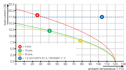
BCZ 3.81../180 - SCD-THR 3.81../180
