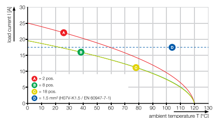
BCF 3.81../180 - SC 3.81../90
