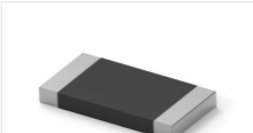
TE Part #6-2176422-2 TLRP 2512 3.0W R033 1% 50PPM 4K RL
