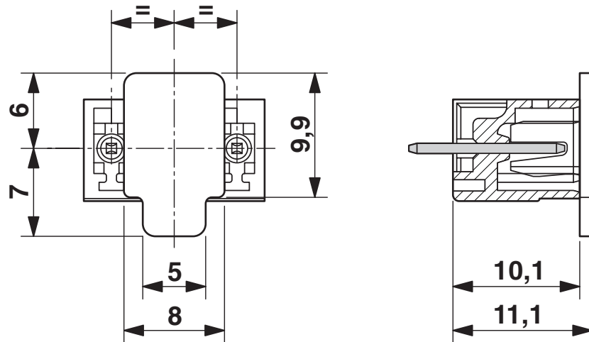
Dimensional drawing
