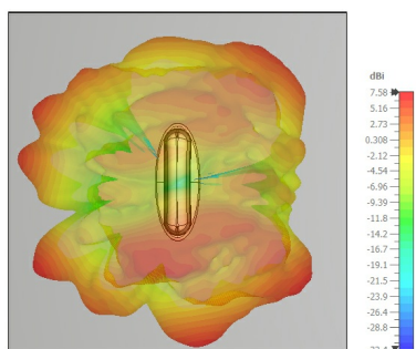
6000 MHz, top view
