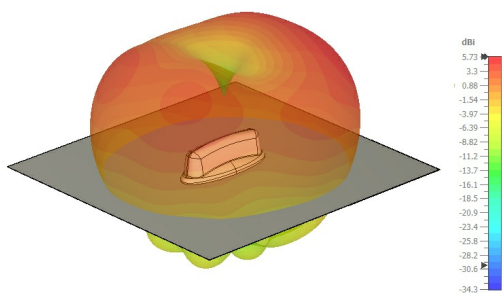
900 MHz, side view
