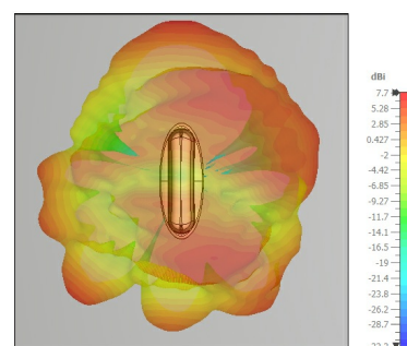
5000 MHz, top view
