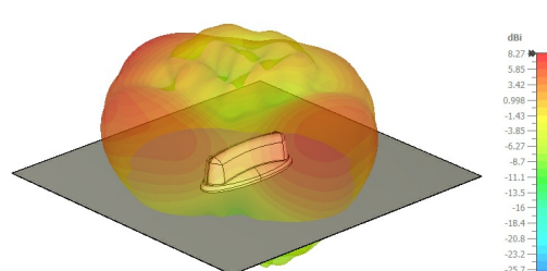
2100 MHz, side view
