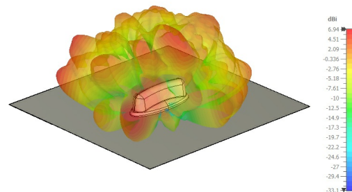
7000 MHz, side view
