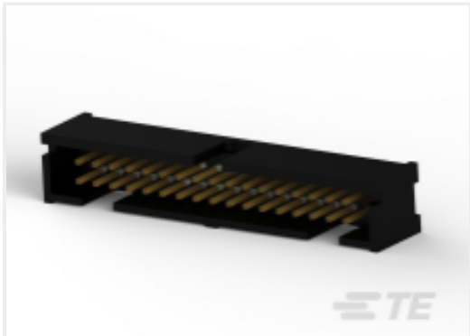
TE Part # 5103310-7 A/L LOW PRO HDR 34P RA BLACK
