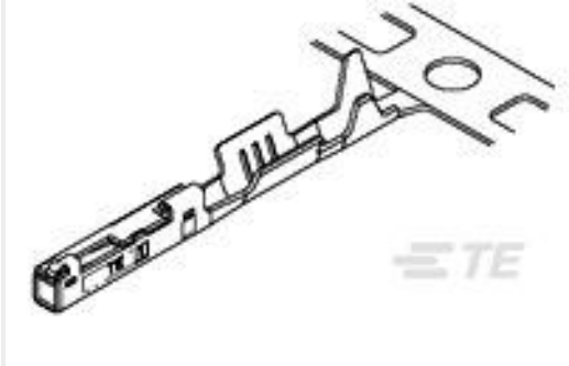
TE Part #1827855-4 0.50 SERIES CONNECTER RECEPTACLE CONTACT
