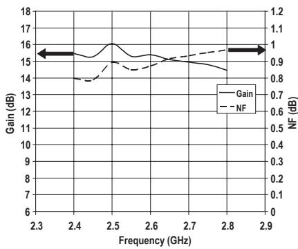
Figure 26. Gain and NF vs Frequency
