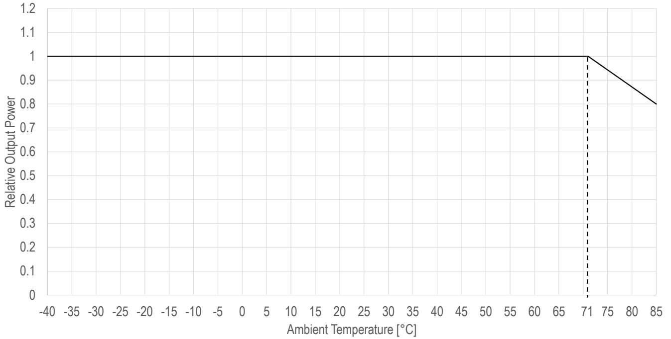
1779405x41 Output Power Thermal Derating Nominal V_{IN} , I_{OUT} = 0.4A
