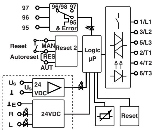
Figure 3 Block diagram
