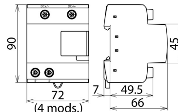
Dimension drawing DCB YPV SCI 600
