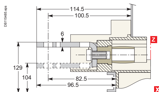
NSX400/630
