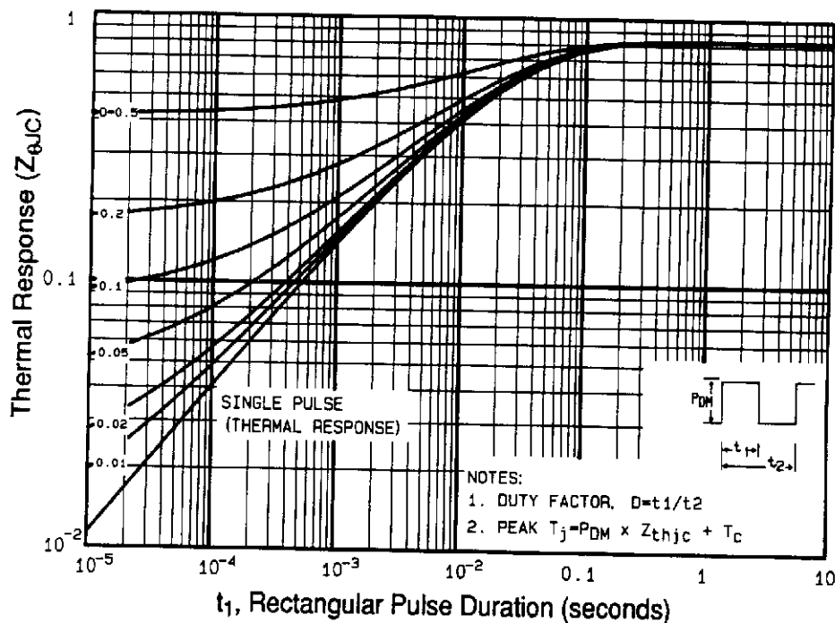
Fig 11. Maximum Effective Transient Thermal Impedance, Junction-to-Case
