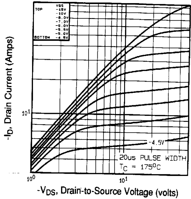
Fig 2. Typical Output Characteristics, T_C = 175^\circ\text{C}
