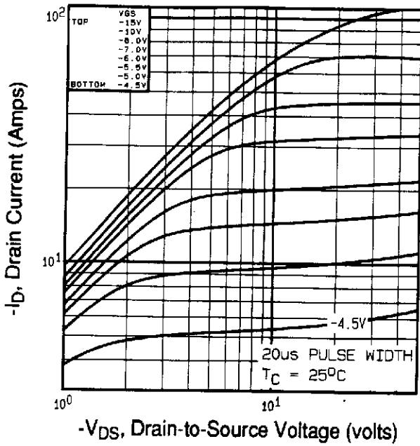
Fig 1. Typical Output Characteristics, T_C = 25^\circ\text{C}
