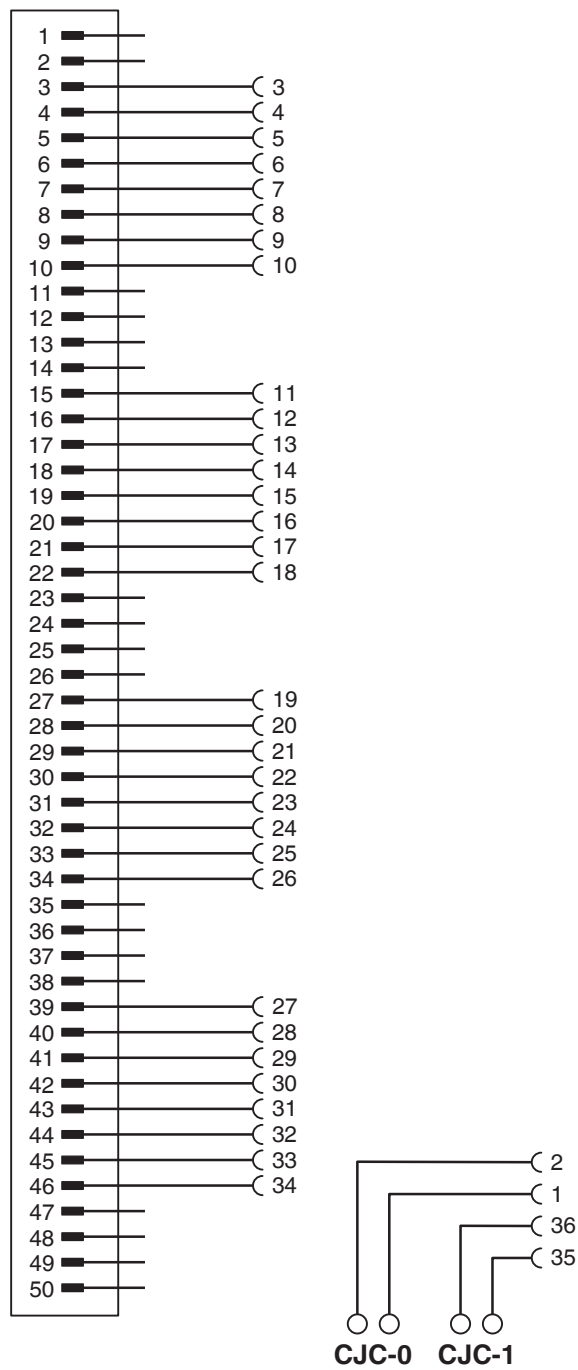
Circuit diagram
