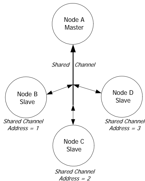
Figure 8-2: Shared channel implementation of example network
