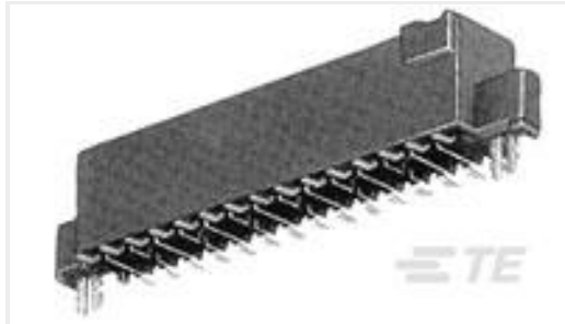
TE Part #147384-3 30 50/50 GRID DR SMT RCPT VC
