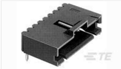
TE Part #1-103634-3 14 MTE HDR SRRA LATCH .100CL
