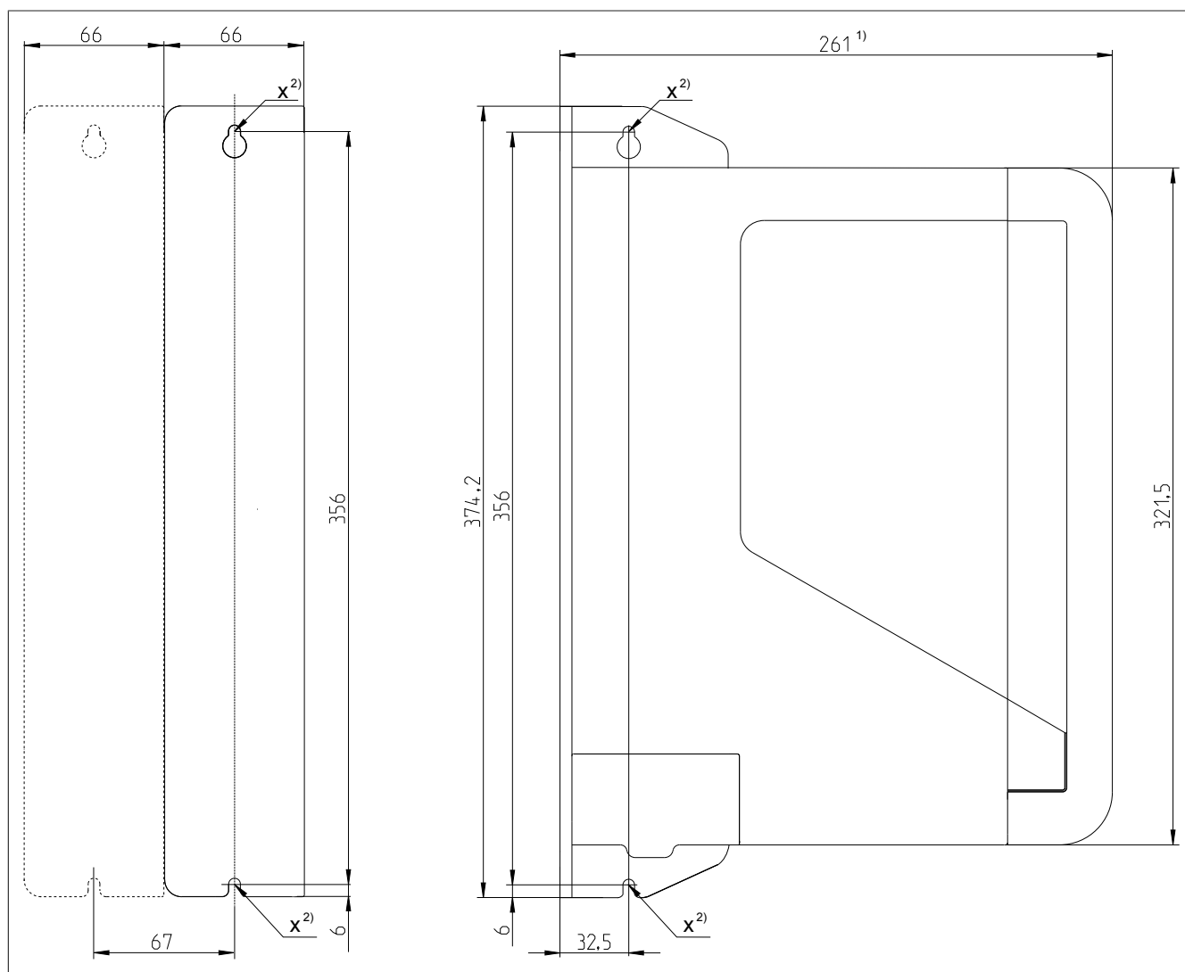
Figure 2: SafeMOTION single-width 2-axis modules - Dimension diagram
