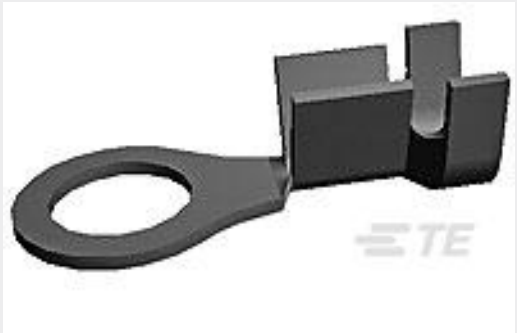
TE Part #42037-2 RING TERMINAL 22-18 AWG TPBR
