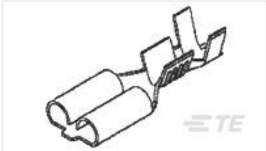
TE Part #170384-1 250 FASTON,REC.,22-20 AWG,BR
