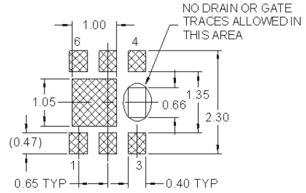
RECOMMENDED LAND PATTERN OPT 1
