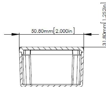
ASSEMBLY
