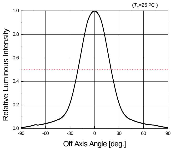
Radiation Diagram
