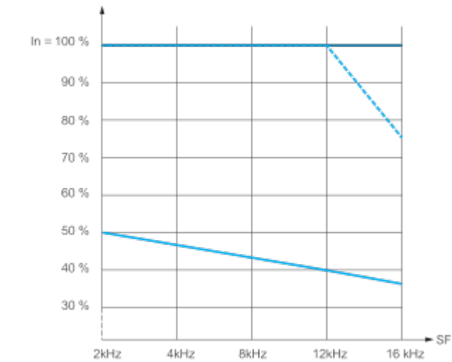
— 40 °C (104 °F) - Mounting type A - - - 50 °C (122 °F) - Mounting type A — 60 °C (140 °F) - Mounting type A In : Nominal Drive Current SF : Switching Frequency
