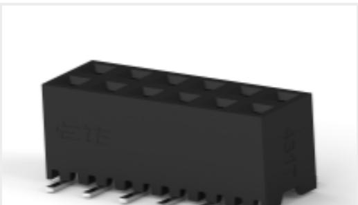
TE Part #1-2314846-2 12P,2MM,BB,REC,DRVT,SMD,AU.76,TB,W/CP
