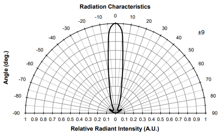
Radiation of single LED (UN)
