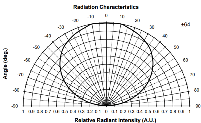
Radiation of single LED (UW)
