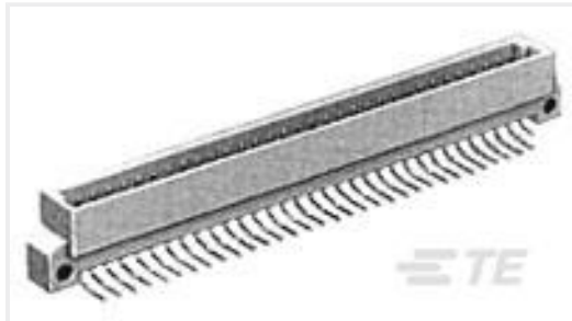
TE Part #5536053-5 ASSY,PIN,EUROCARD,TYPE B/2,LEA
