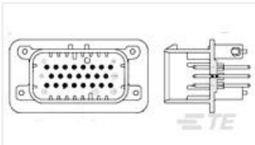
TE Part #776228-2 23POS,PIN DIA 1.3,HDR ASSY, 180DEG,COD 2
