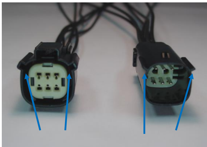
Keying features
