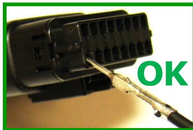
Orientation Feature
