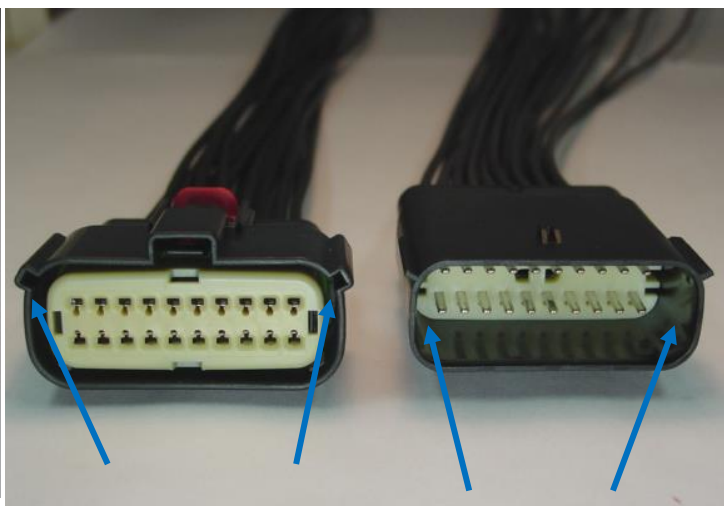
Keying Features
