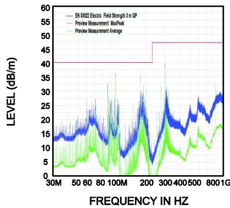
Radiated EMI
