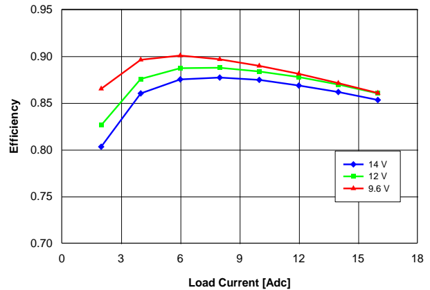
Fig. 1.5V.2: Efficiency vs. load current and input voltage for V_{out} = 1.5V converter mounted vertically with air flowing at a rate of 200 LFM (1 m/s) and T_a = 25^{\circ}C .
