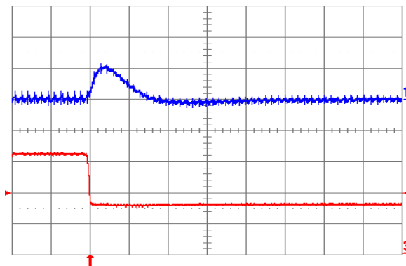
Fig. 2.5V.7: Output voltage response for V_{out} = 2.5V to negative load current step change from 16A to 8A with slew rate of -5A/ \mu s at V_{in} = 12V . Top trace: output voltage (200mV/div.); Bottom trace: load current (5A/div.). C_o = 100\mu F ceramic. Time scale: 20 \mu s /div.
