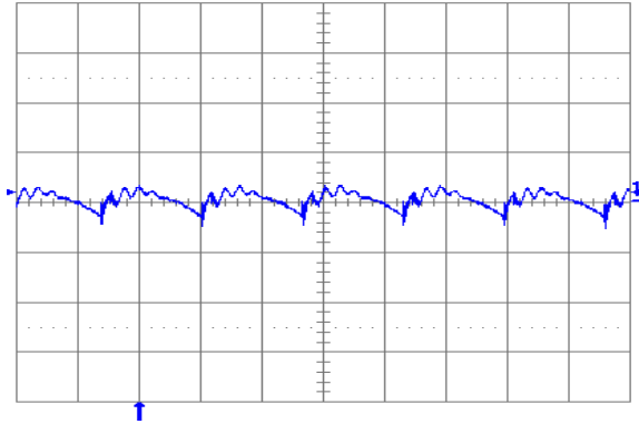
Fig. 1.0V.5: Output voltage ripple (20mV/div.) at full rated load current into a resistive load with external capacitance 100µF ceramic + 1µF ceramic and V_{in} = 12V for V_{out} = 1.0V . Time scale: 2µs/div.
