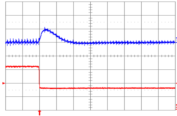
Fig. 1.8V.7: Output voltage response for V_{out} = 1.8V to negative load current step change from 16A to 8A with slew rate of -5A/ \mu s at V_{in} = 12V . Top trace: output voltage (200mV/div.); Bottom trace: load current (5A/div.). C_o = 100\mu F ceramic. Time scale: 20 \mu s/div.
