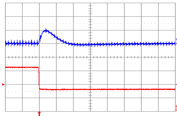
Fig. 1.5V.7: Output voltage response for V_{out} = 1.5V to negative load current step change from 16A to 8A with slew rate of -5A/\mu s at V_{in} = 12V . Top trace: output voltage (200mV/div.); Bottom trace: load current (5A/div.). C_o = 100\mu F ceramic. Time scale: 20μs/div.
