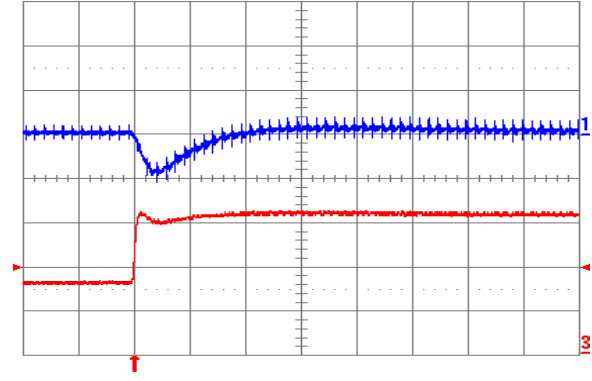
Fig. 1.0V.6: Output voltage response for V_{out} = 1.0V to positive load current step change from 8A to 16A with slew rate of 5A/µs at V_{in} = 12V . Top trace: output voltage (200mV/div.); Bottom trace: load current (5A/div.). C_o = 100µF ceramic. Time scale: 20µs/div.
