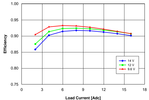
Fig. 2.5V.2: Efficiency vs. load current and input voltage for V_{out} = 2.5V converter mounted vertically with air flowing at a rate of 200 LFM (1 m/s) and T_a = 25^{\circ}C .
