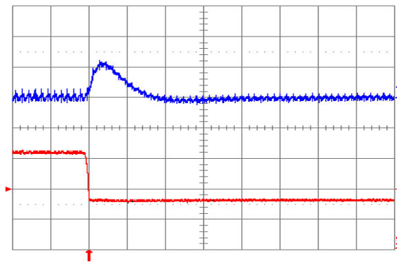
Fig. 3.3V.7: Output voltage response for V_{out} = 3.3V to negative load current step change from 16A to 8A with slew rate of -5A/ \mu s at V_{in} = 12V . Top trace: output voltage (200mV/div.); Bottom trace: load current (5A/div.). C_o = 100\mu F ceramic. Time scale: 20 \mu s/div.
