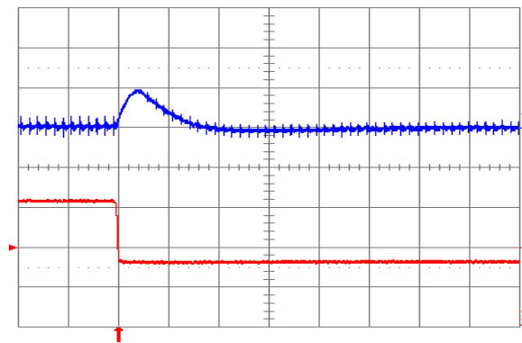
Fig. 1.0V.7: Output voltage response for V_{out} = 1.0V to negative load current step change from 16A to 8A with slew rate of -5A/µs at V_{in} = 12V . Top trace: output voltage (200mV/div.); Bottom trace: load current (5A/div.). C_o = 100µF ceramic. Time scale: 20µs/div.
