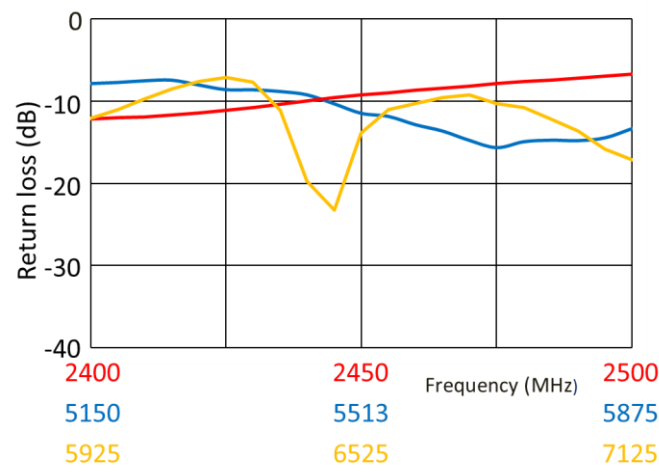
Return Loss
