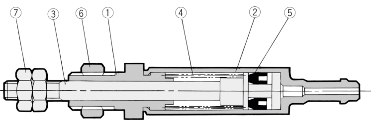
CJ1B4-□SU4
